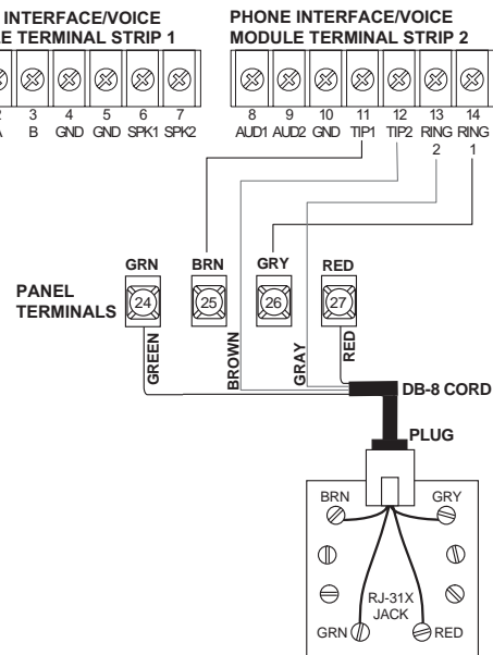
Figure 8. Wiring the PIV to a Phone Line (Partition 1)
