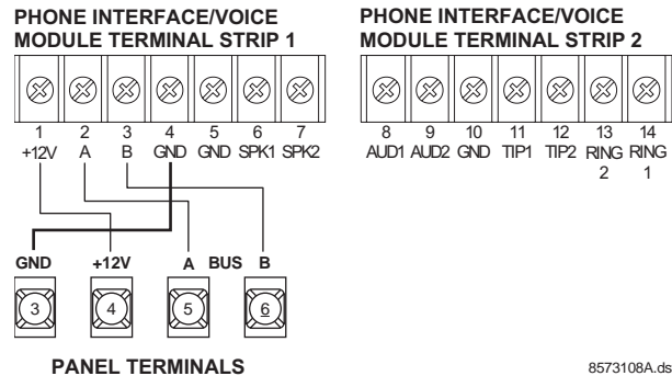
PANEL TERMINALS
